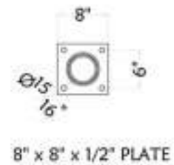
4" Steel Bollard with Cover
