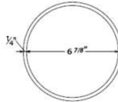
Cross Section of Sleeve
